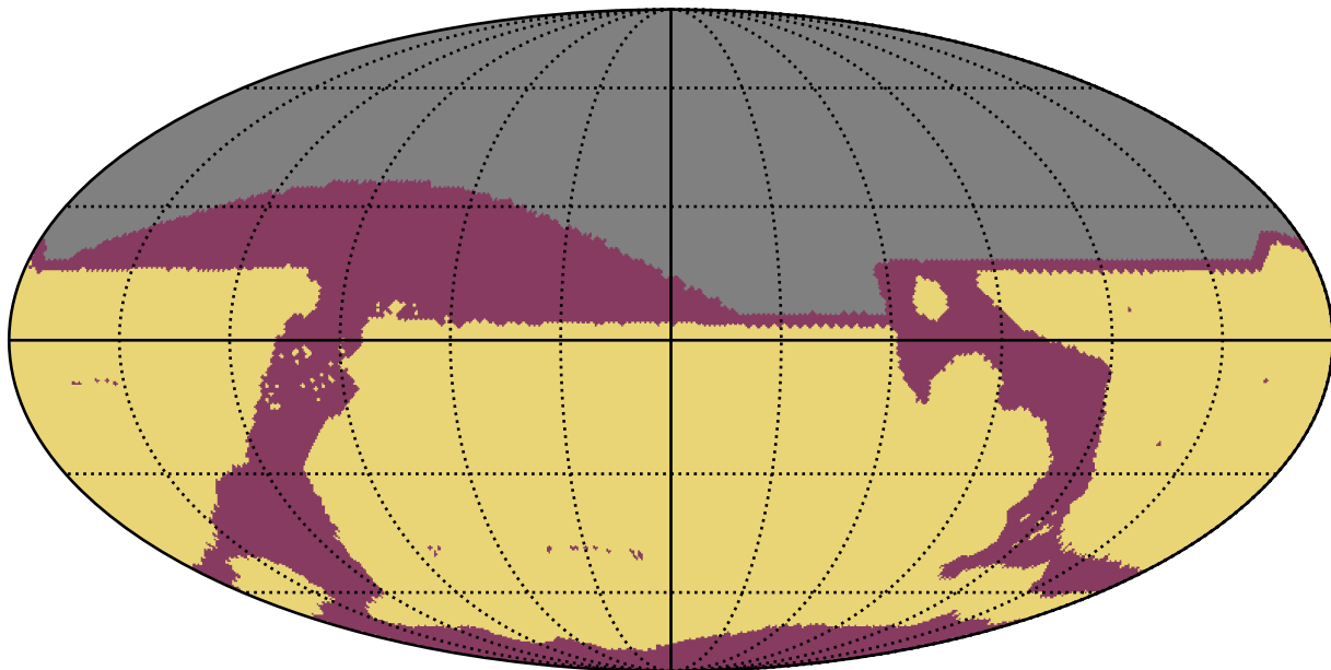
early_u_fpextra3.0_v3.4_10yrs : RapidRevisits
