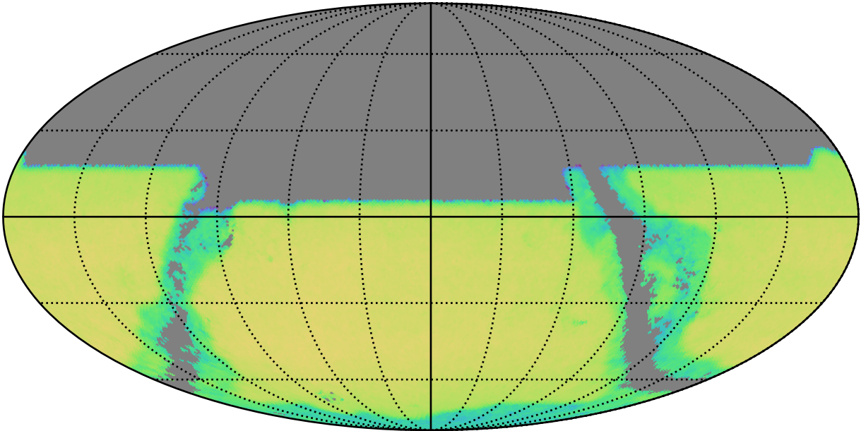
early_u_fpextra3.0_v3.4_10yrs y band and non-DD: QSONumberCountsMetric
