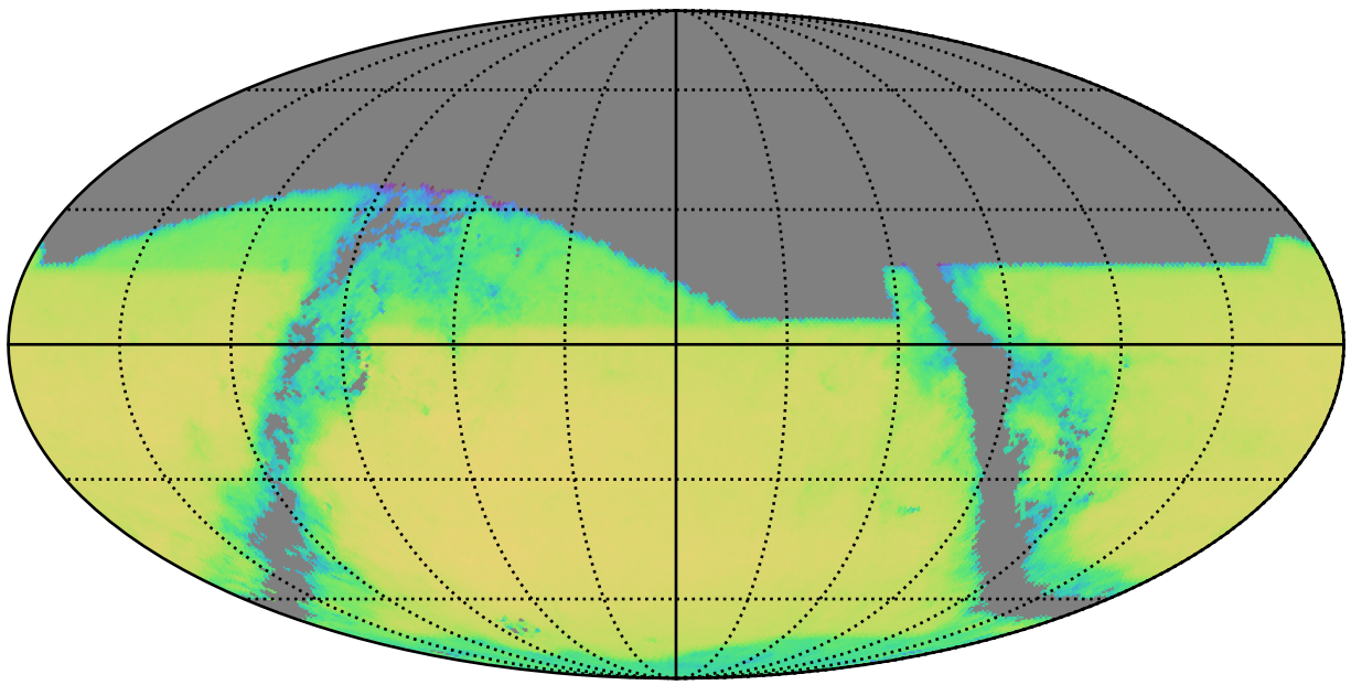
early_u_fpextra3.0_v3.4_10yrs r band and non-DD: QSONumberCountsMetric
