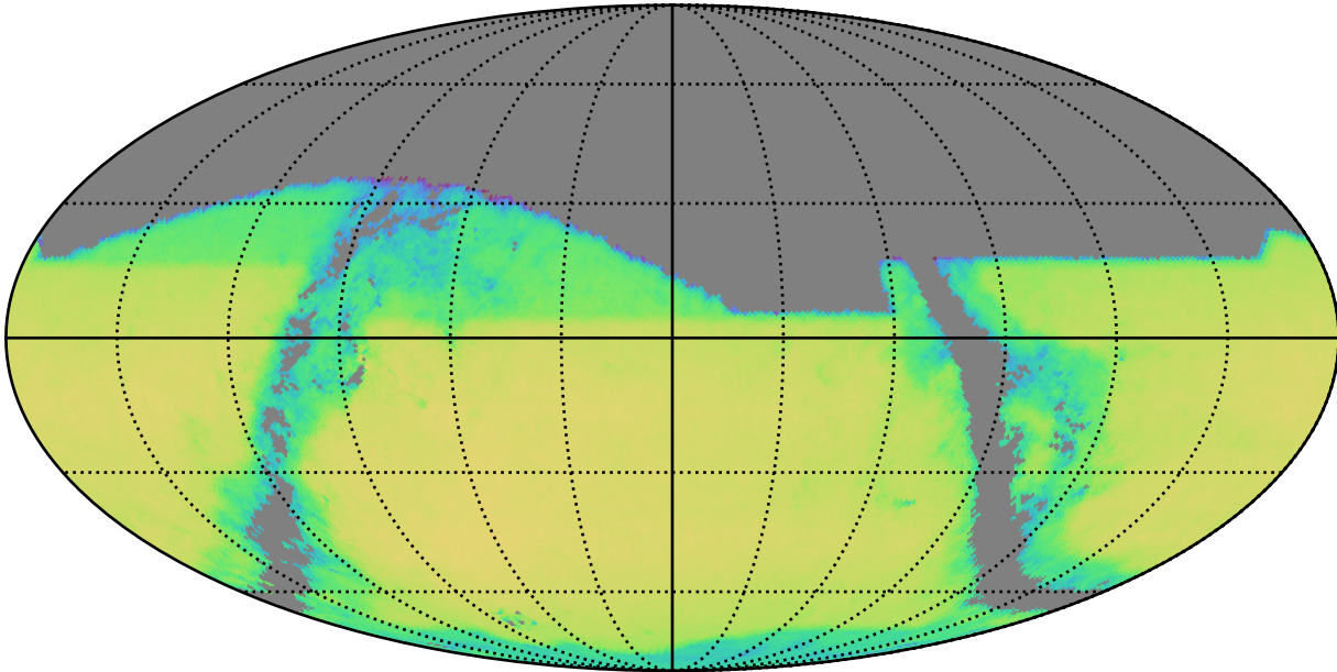
early_u_fpextra3.0_v3.4_10yrs i band and non-DD: QSONumberCountsMetric
