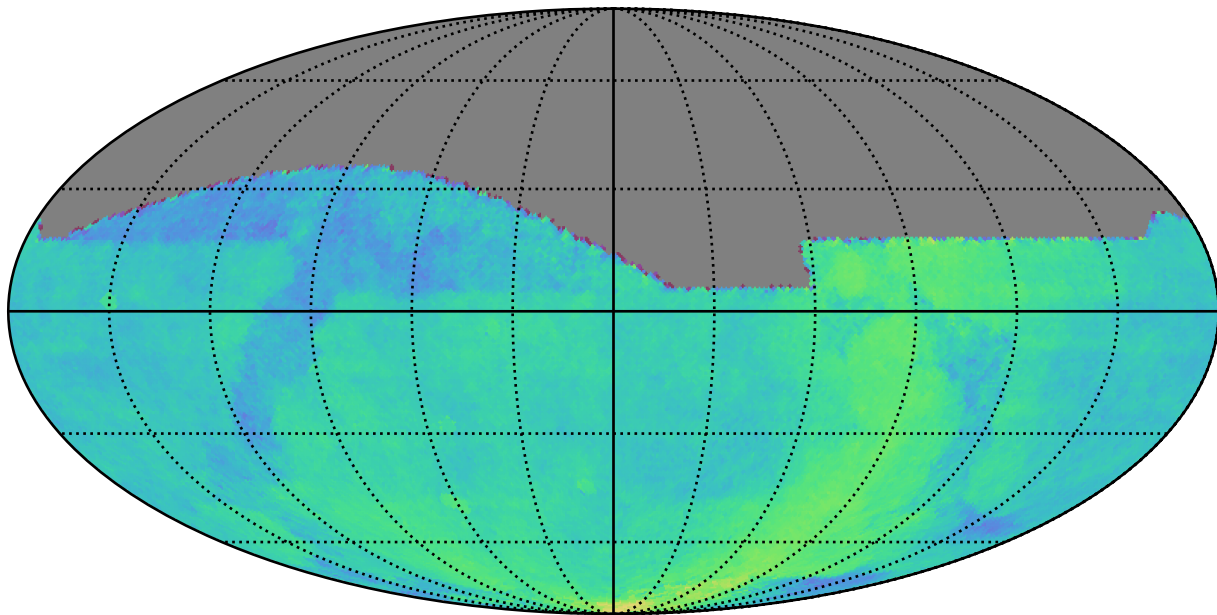
early_u_fpextra3.0_v3.4_10yrs : Parallax Coverage @ 22.4
