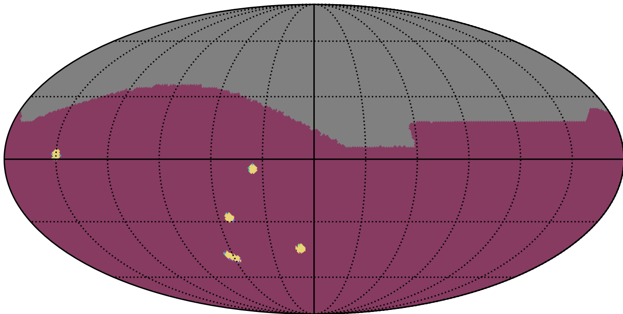
early_u_fpextra3.0_v3.4_10yrs : NumberOfQuickRevisits
