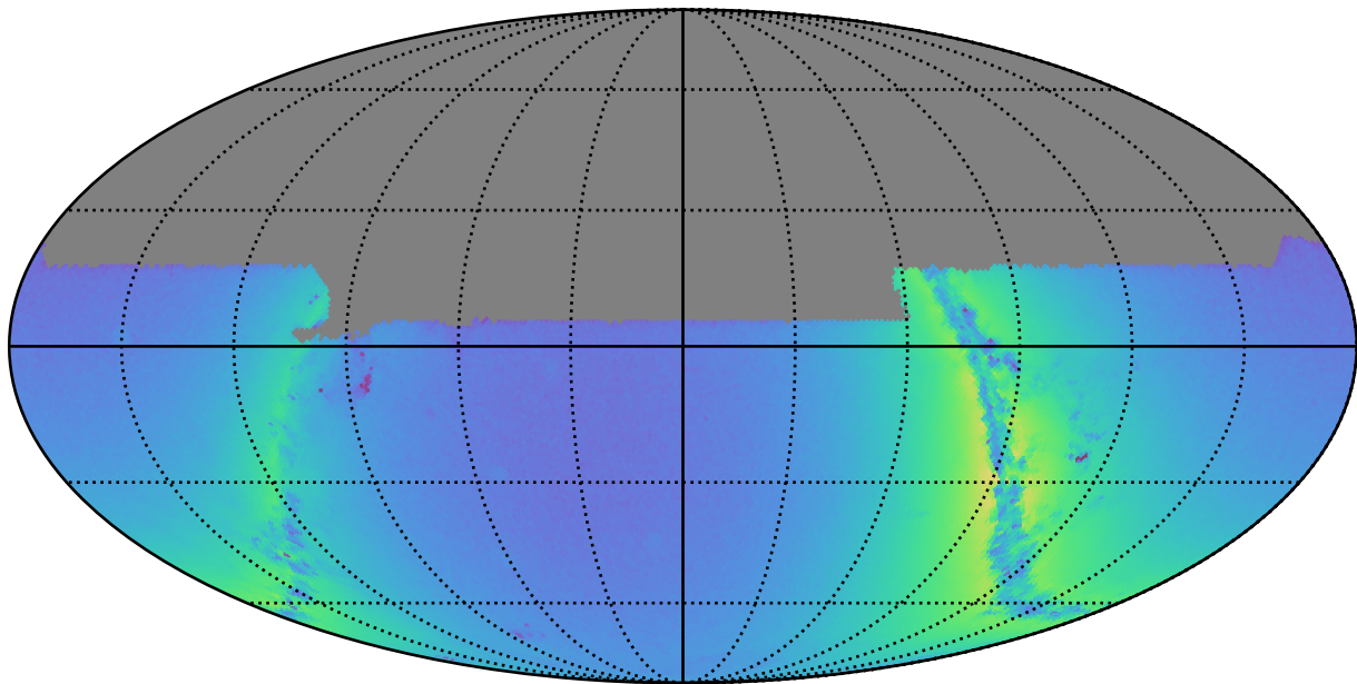
early_u_fpextra3.0_v3.4_10yrs u: Nstars_no_crowding
