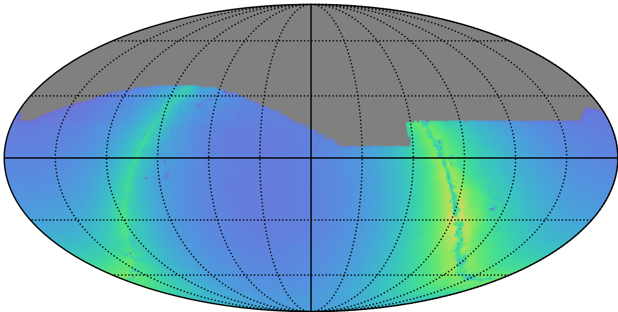
early_u_fpextra3.0_v3.4_10yrs r: Nstars_no_crowding
