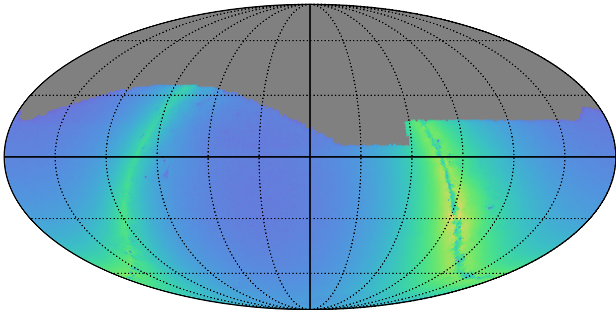
early_u_fpextra3.0_v3.4_10yrs i: Nstars_no_crowding
