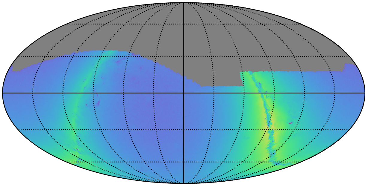
early_u_fpextra3.0_v3.4_10yrs g: Nstars_no_crowding
