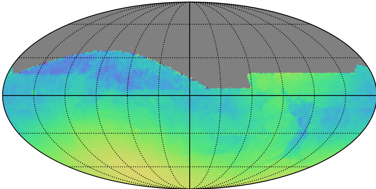
early_u_fpextra3.0_v3.4_10yrs : Normalized Parallax Uncert @ 24.0
