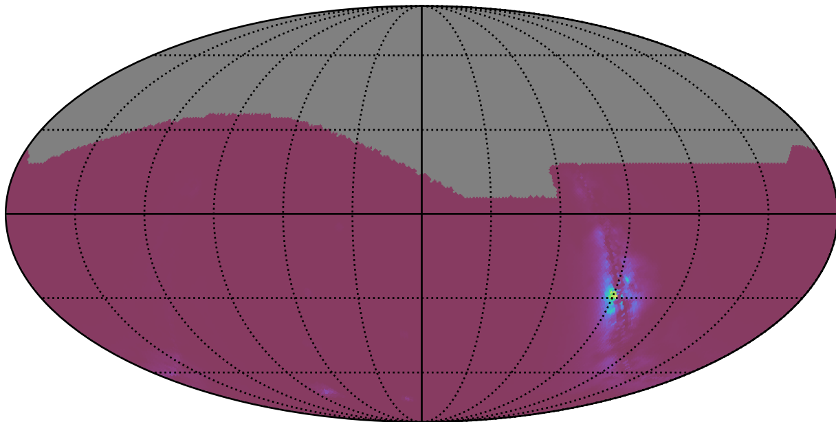
early_u_fpextra3.0_v3.4_10yrs : NlcPoints
