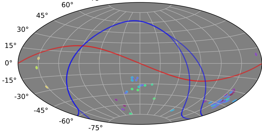
early_u_fpextra3.0_v3.4_10yrs gi: LVDwarfs 75°
