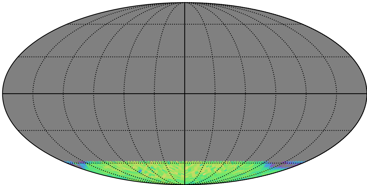
early_u_fpextra3.0_v3.4_10yrs gi SCP: LVDwarfs
