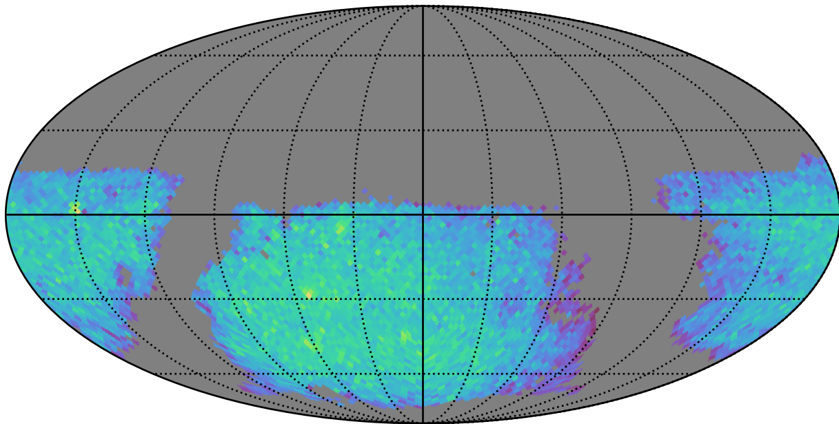
early_u_fpextra3.0_v3.4_10yrs gi: LVDwarfs
