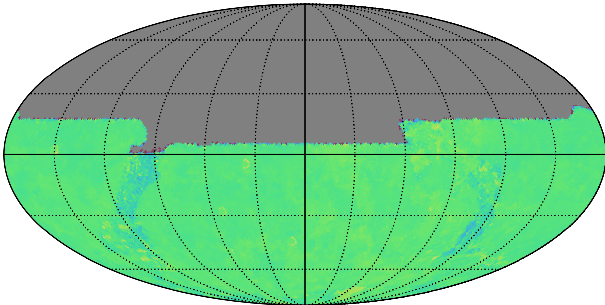
early_u_fpextra3.0_v3.4_10yrs u: Kuiper rotTelPos
