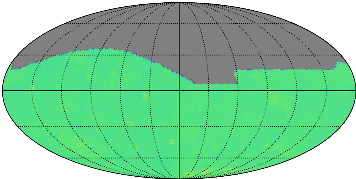
early_u_fpextra3.0_v3.4_10yrs r: Kuiper rotTelPos
