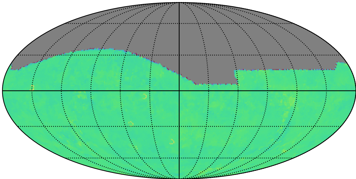
early_u_fpextra3.0_v3.4_10yrs g: Kuiper rotTelPos
