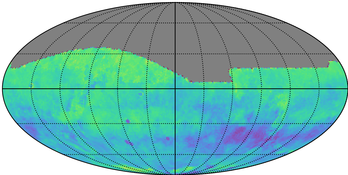
early_u_fpextra3.0_v3.4_10yrs z: Kuiper rotSkyPos
