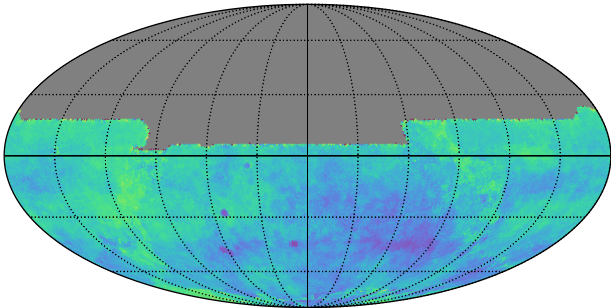
early_u_fpextra3.0_v3.4_10yrs y: Kuiper rotSkyPos
