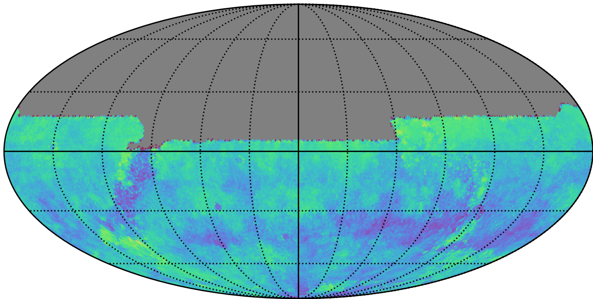
early_u_fpextra3.0_v3.4_10yrs u: Kuiper rotSkyPos
