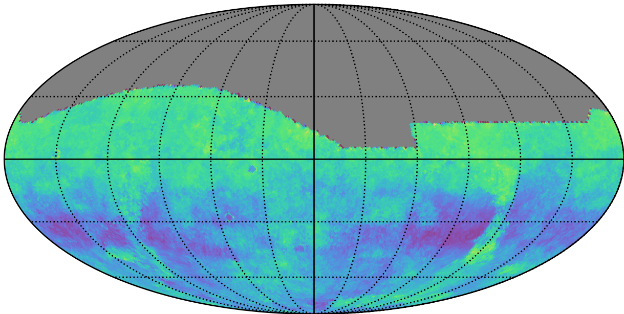
early_u_fpextra3.0_v3.4_10yrs g: Kuiper rotSkyPos
