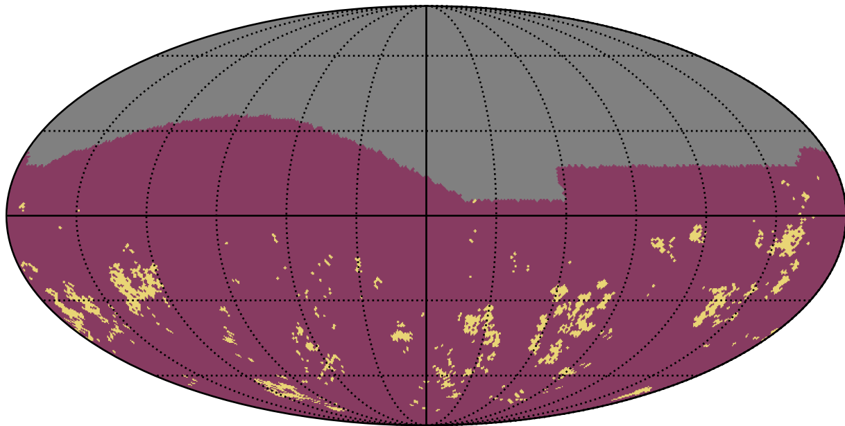
early_u_fpextra3.0_v3.4_10yrs g band: Gaps_7hr
