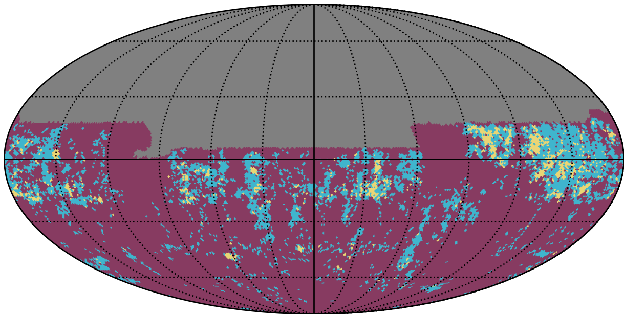
early_u_fpextra3.0_v3.4_10yrs u band: Gaps_3hr
