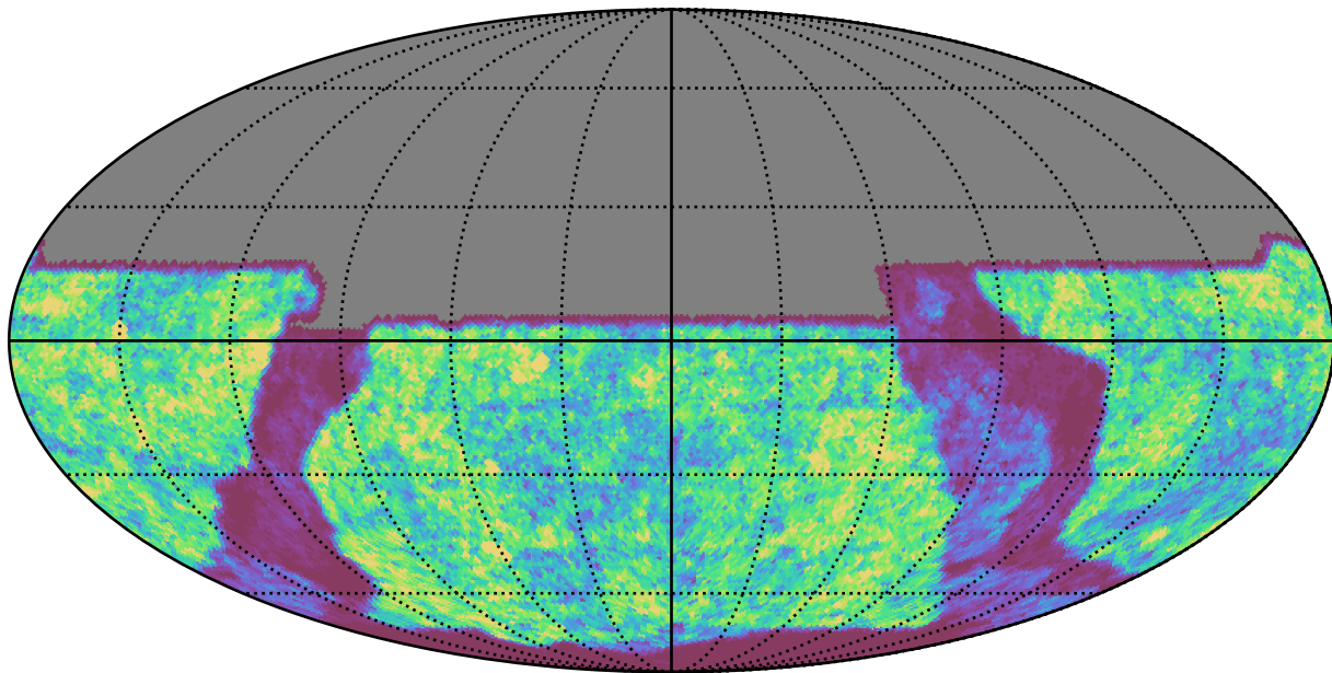
early_u_fpextra3.0_v3.4_10yrs y band: Gaps_24hr
