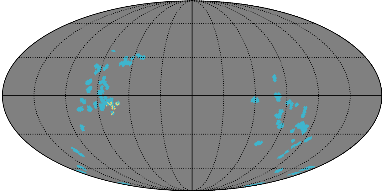
early_u_fpextra3.0_v3.4_10yrs : GalplaneFootprintMetric_zucker_sfr_map_Tau_5_0
