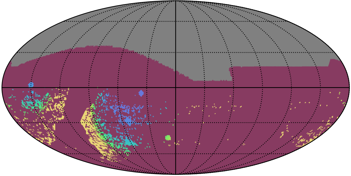
early_u_fpextra3.0_v3.4_10yrs : GalplaneFootprintMetric_xray_binaries_map_Tau_5_0
