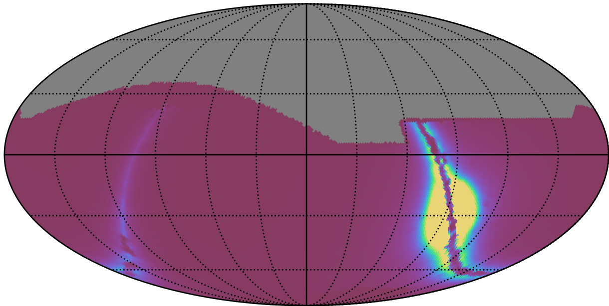
early_u_fpextra3.0_v3.4_10yrs : GalplaneFootprintMetric_xray_binaries_map_Tau_46_5
