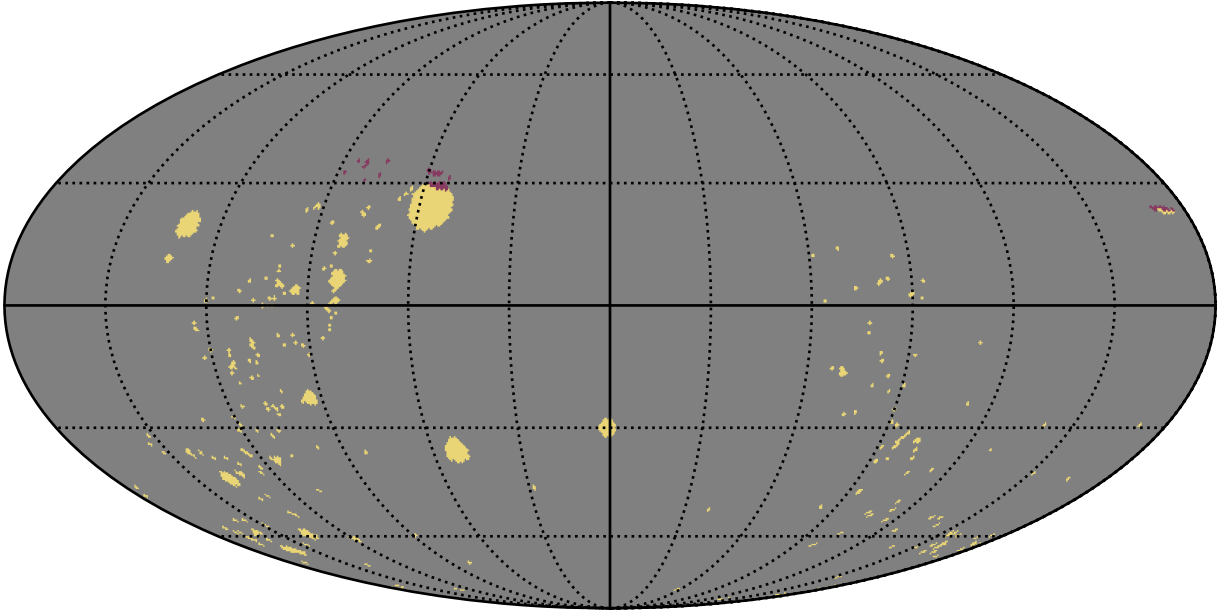
early_u_fpextra3.0_v3.4_10yrs : GalplaneFootprintMetric_open_clusters_map_Tau_73_0
