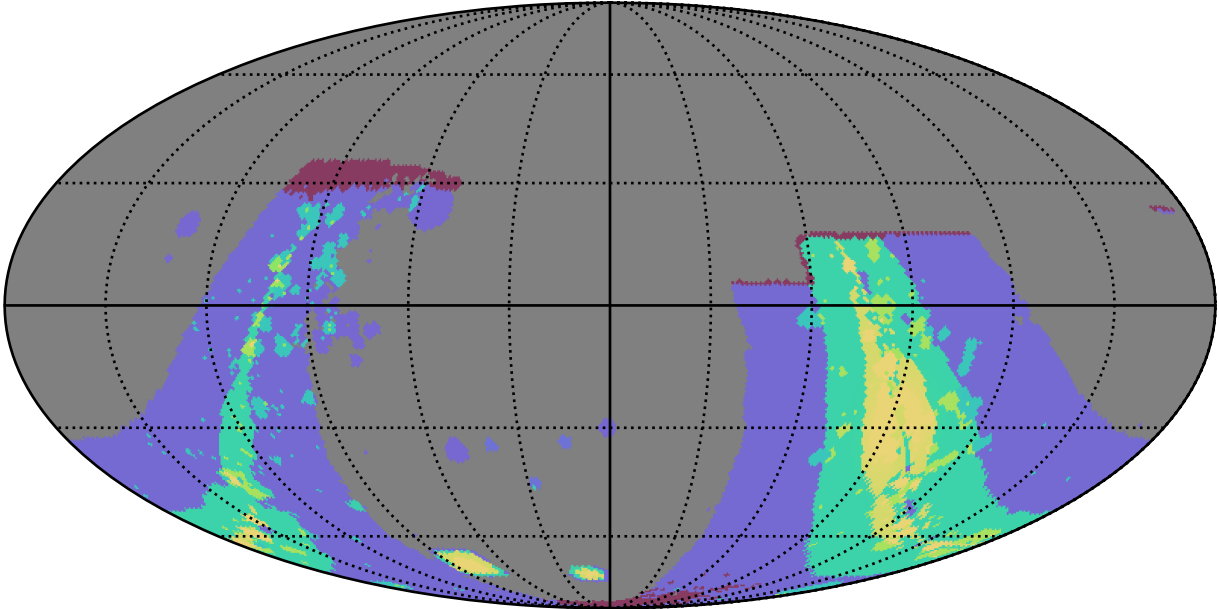
early_u_fpextra3.0_v3.4_10yrs : GalplaneFootprintMetric_combined_map_Tau_73_0
