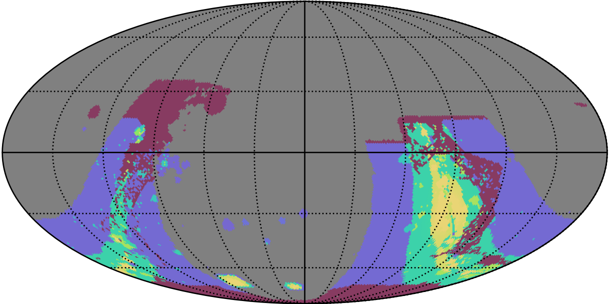
early_u_fpextra3.0_v3.4_10yrs : GalplaneFootprintMetric_combined_map_Tau_20_0
