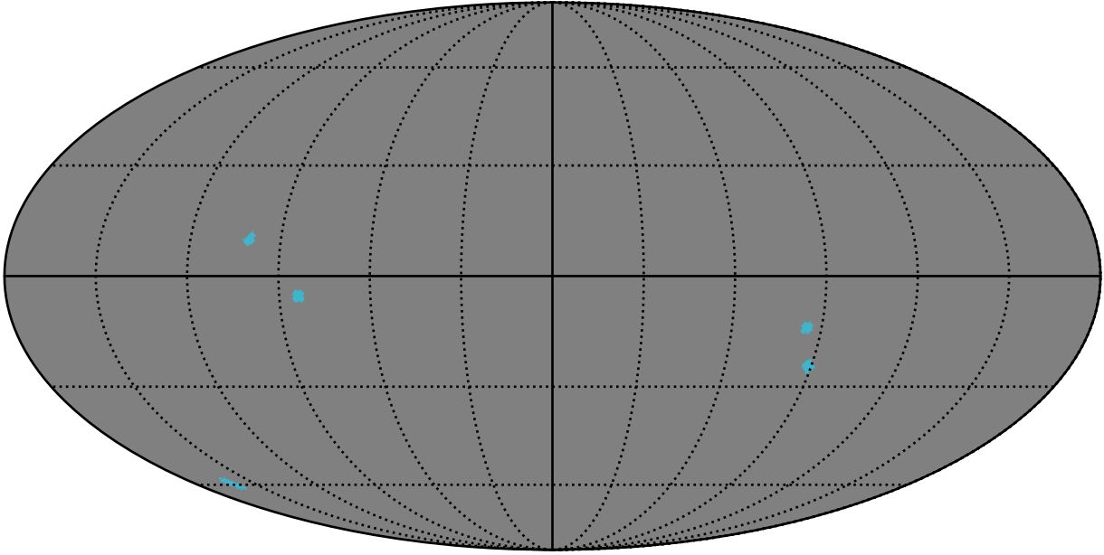
early_u_fpextra3.0_v3.4_10yrs : GalplaneFootprintMetric_bonito_sfr_map_Tau_20_0
