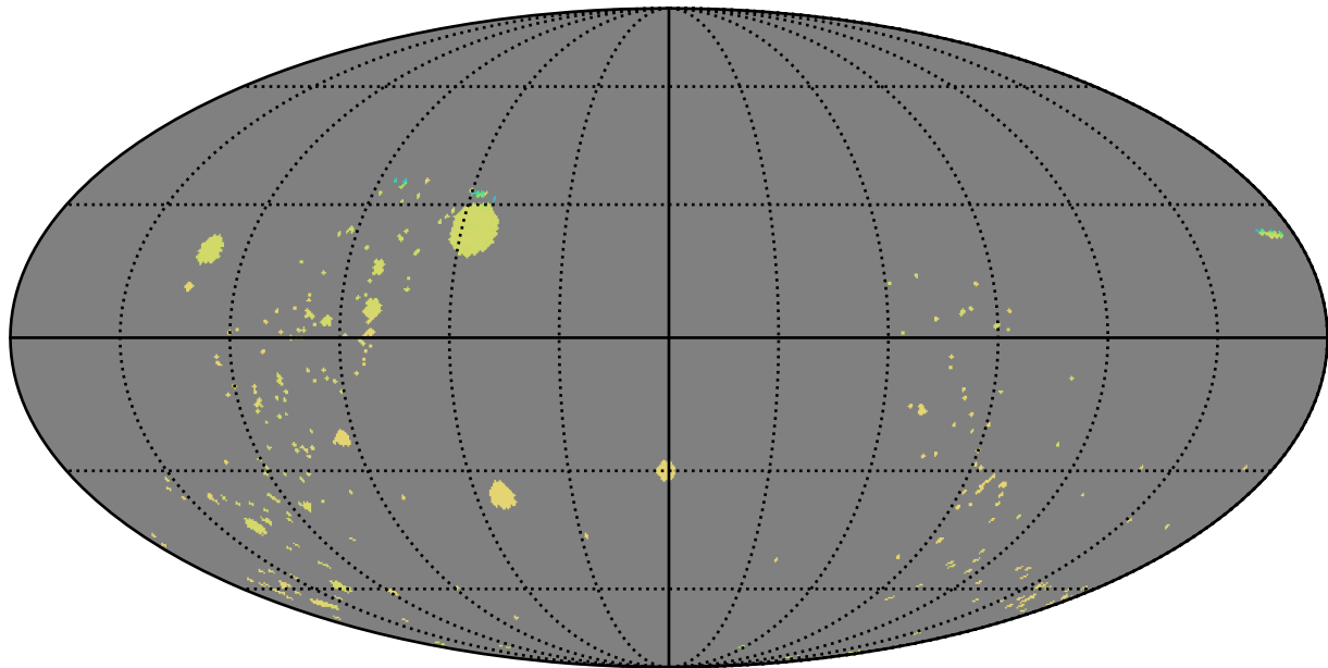
early_u_fpextra3.0_v3.4_10yrs : GalPlaneVisitIntervalsTimescales_open_clusters_map_Tau_73_0
