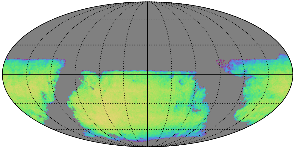
early_u_fpextra3.0_v3.4_10yrs i band galaxies non-DD: DepthLimitedNumGalaxiesMetric
