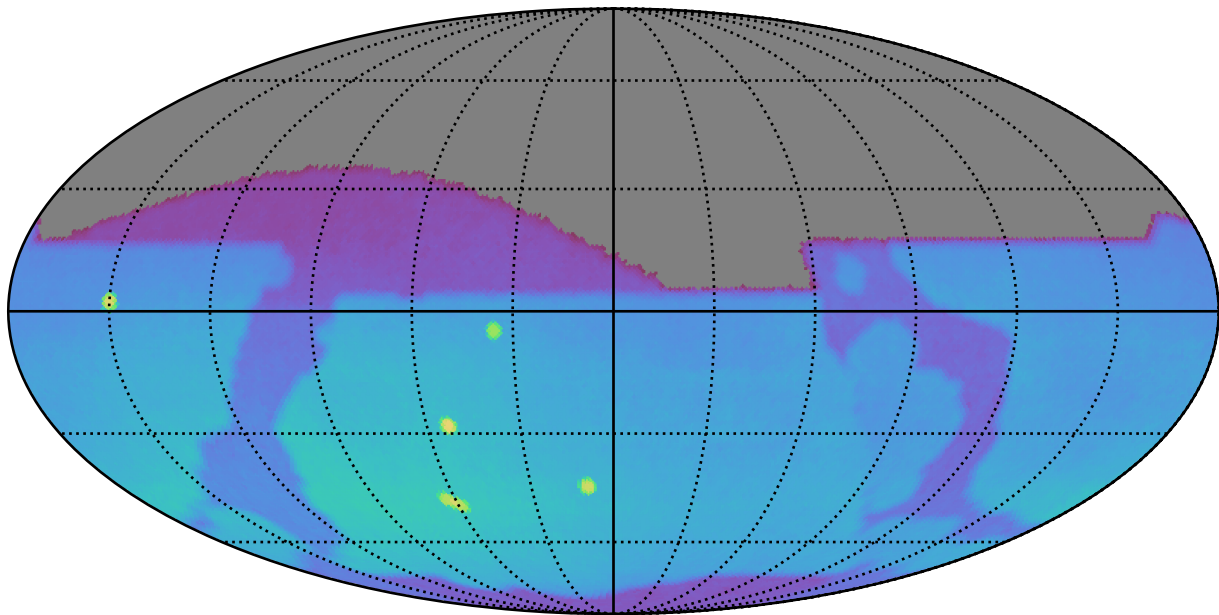
early_u_fpextra3.0_v3.4_10yrs : Brown Dwarf, L4
