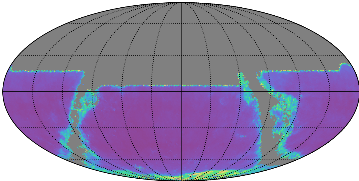
early_u_fpextra3.0_v3.4_10yrs y band: AGN SF_uncert
