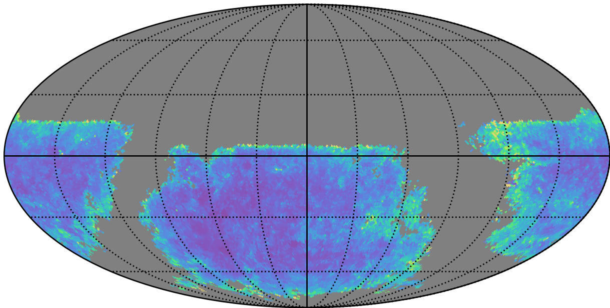
early_u_fpextra3.0_v3.4_10yrs u band: AGN SF_uncert
