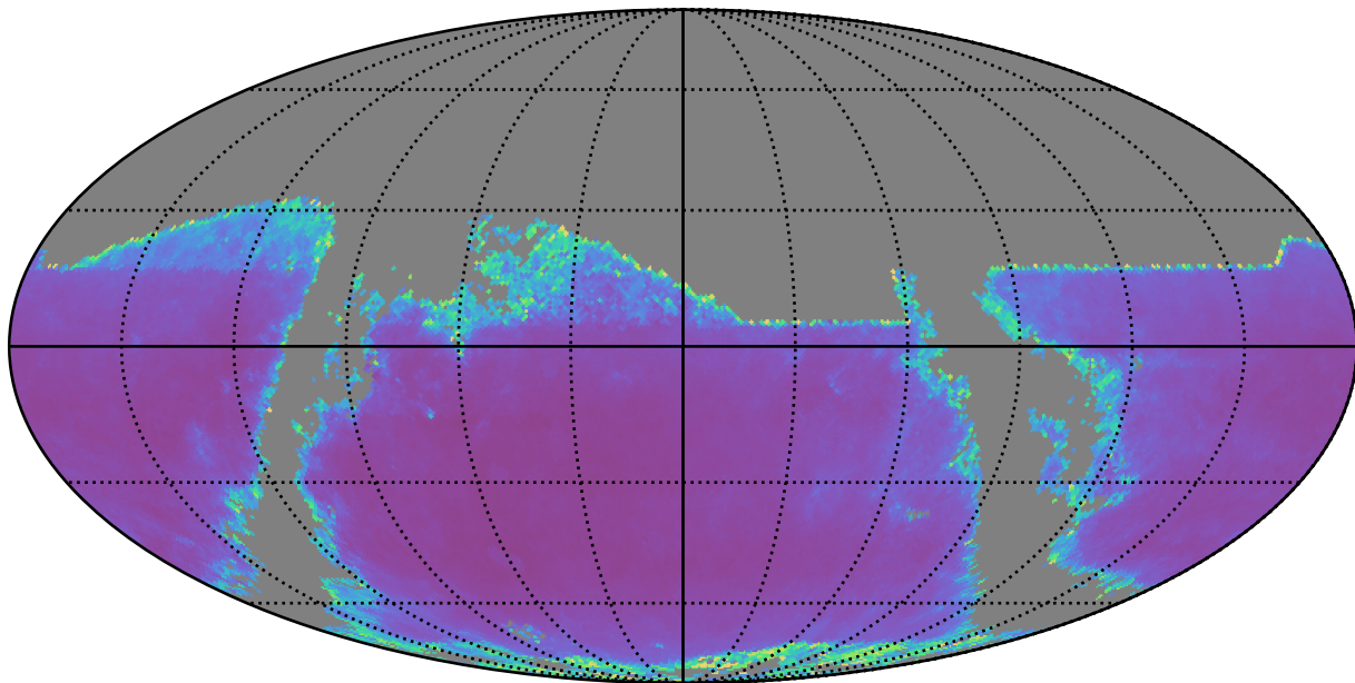
early_u_fpextra3.0_v3.4_10yrs r band: AGN SF_uncert
