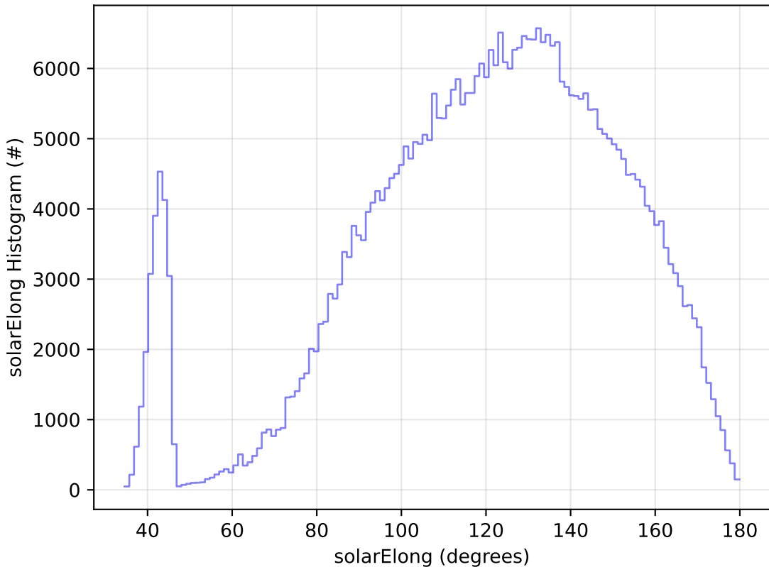
early_u_fpextra3.0_v3.4_10yrs WFD z band: solarElong Histogram
