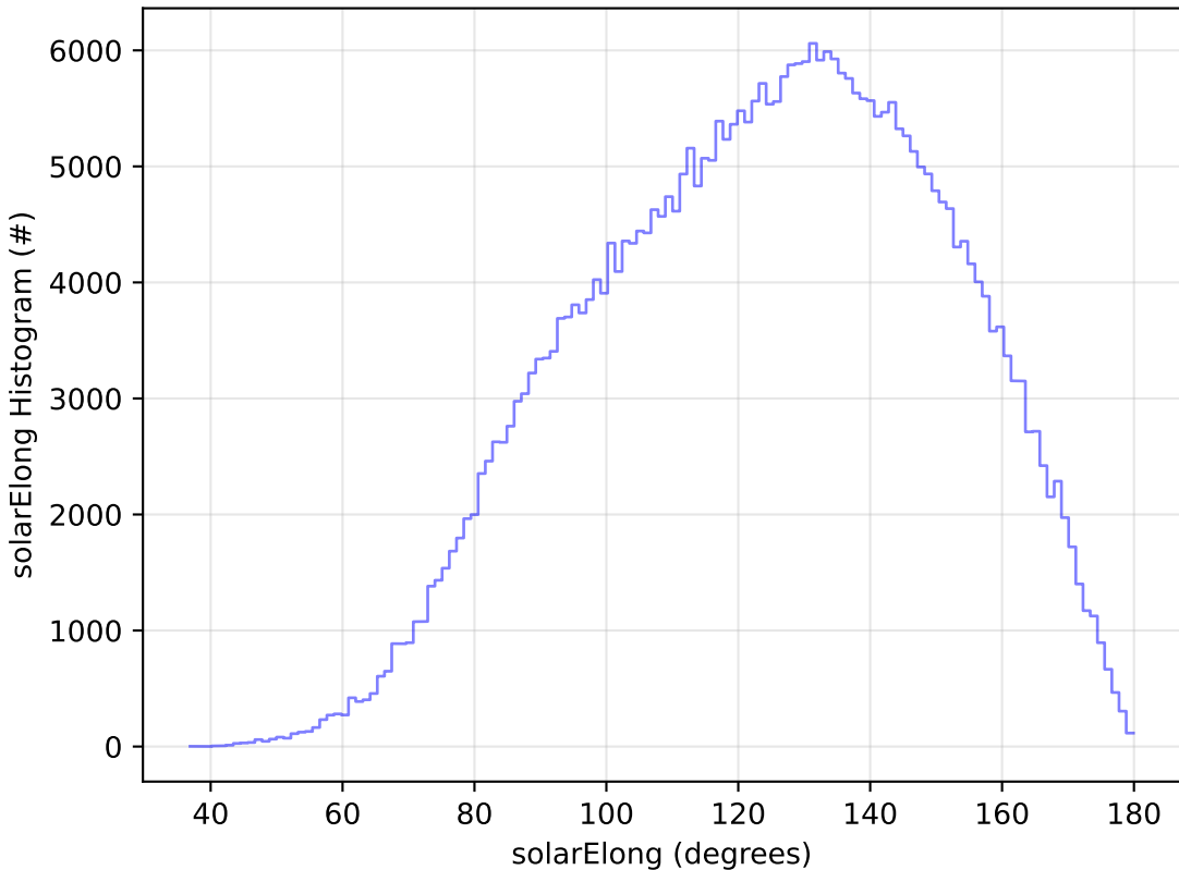
early_u_fpextra3.0_v3.4_10yrs WFD y band: solarElong Histogram
