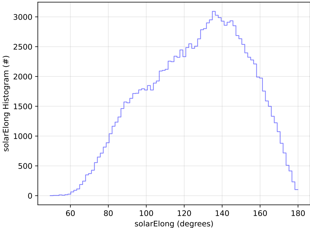
early_u_fpextra3.0_v3.4_10yrs WFD u band: solarElong Histogram
