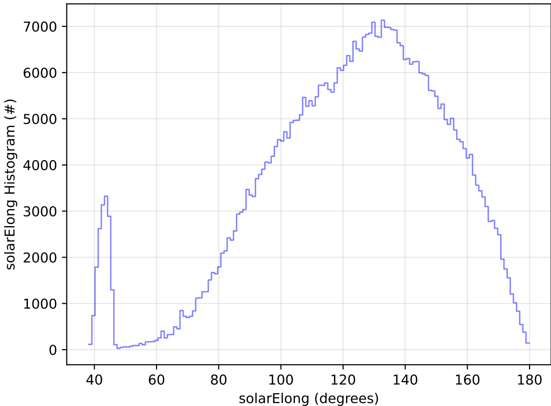
early_u_fpextra3.0_v3.4_10yrs WFD r band: solarElong Histogram
