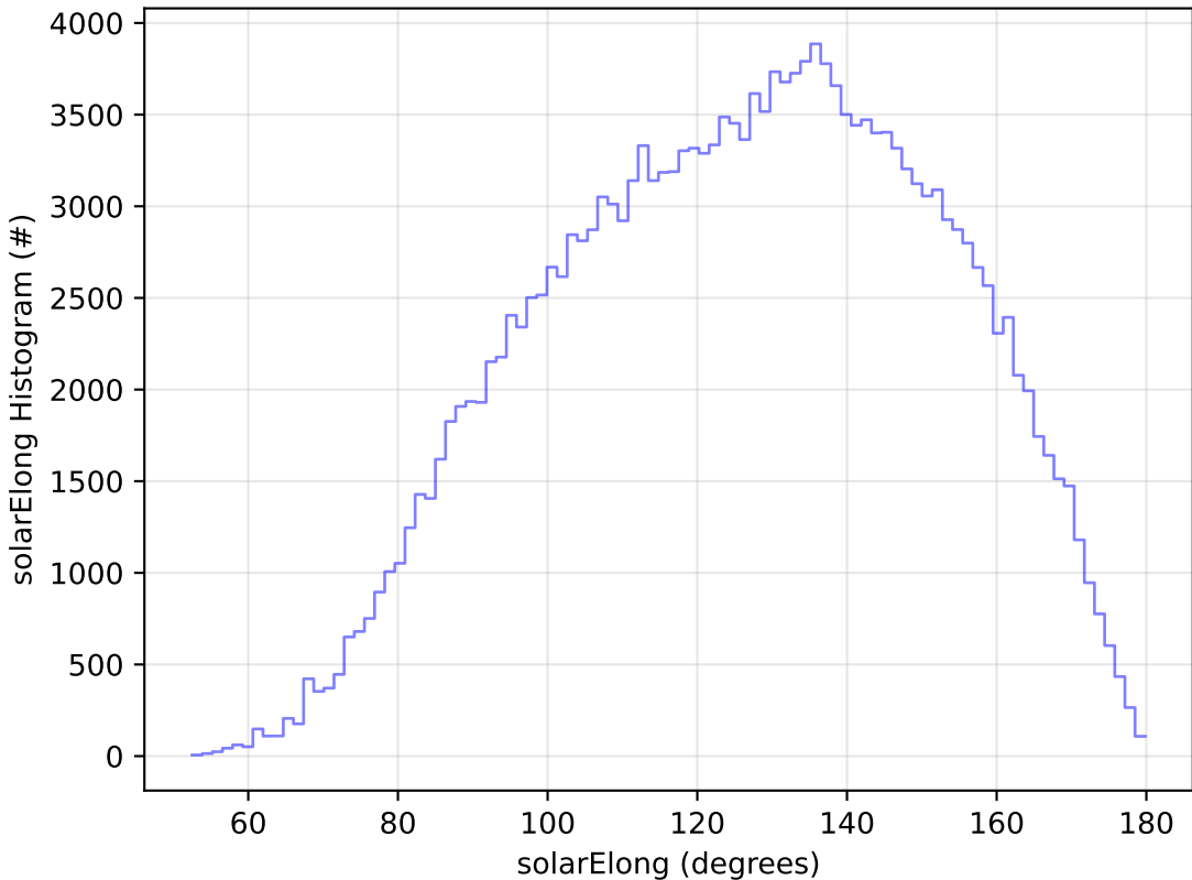
early_u_fpextra3.0_v3.4_10yrs WFD g band: solarElong Histogram
