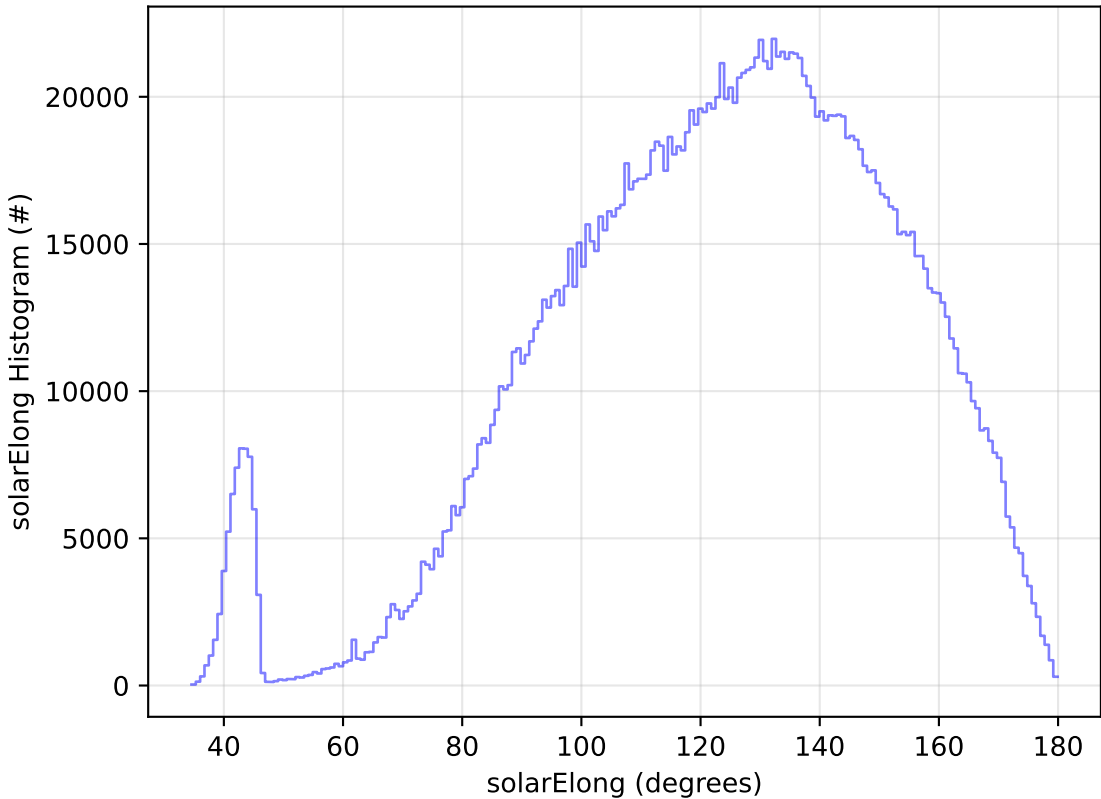
early_u_fpextra3.0_v3.4_10yrs WFD all bands: solarElong Histogram
