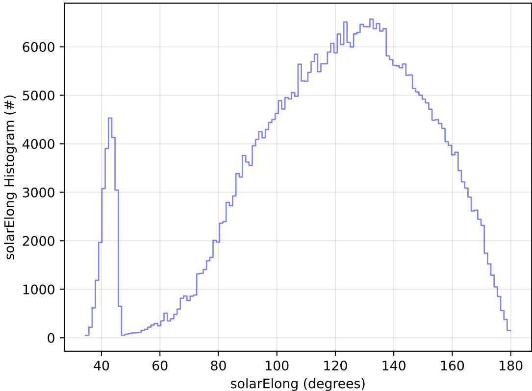
early_u_fpextra3.0_v3.4_10yrs All sky z band: solarElong Histogram
