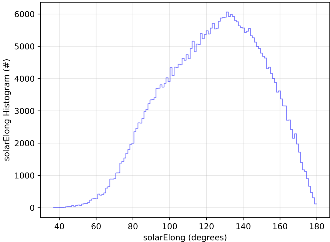
early_u_fpextra3.0_v3.4_10yrs All sky y band: solarElong Histogram
