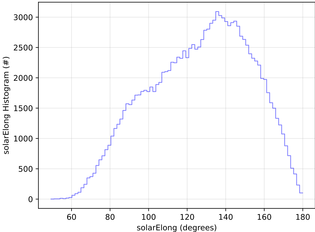
early_u_fpextra3.0_v3.4_10yrs All sky u band: solarElong Histogram
