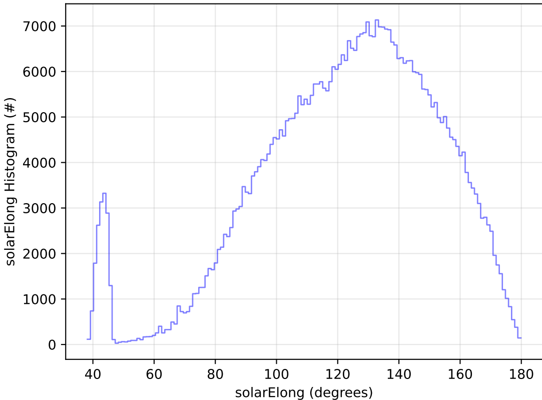
early_u_fpextra3.0_v3.4_10yrs All sky r band: solarElong Histogram
