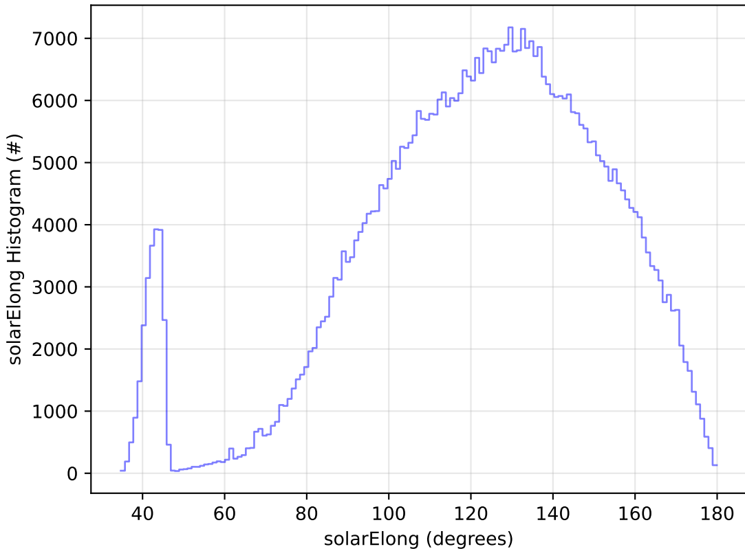
early_u_fpextra3.0_v3.4_10yrs All sky i band: solarElong Histogram
