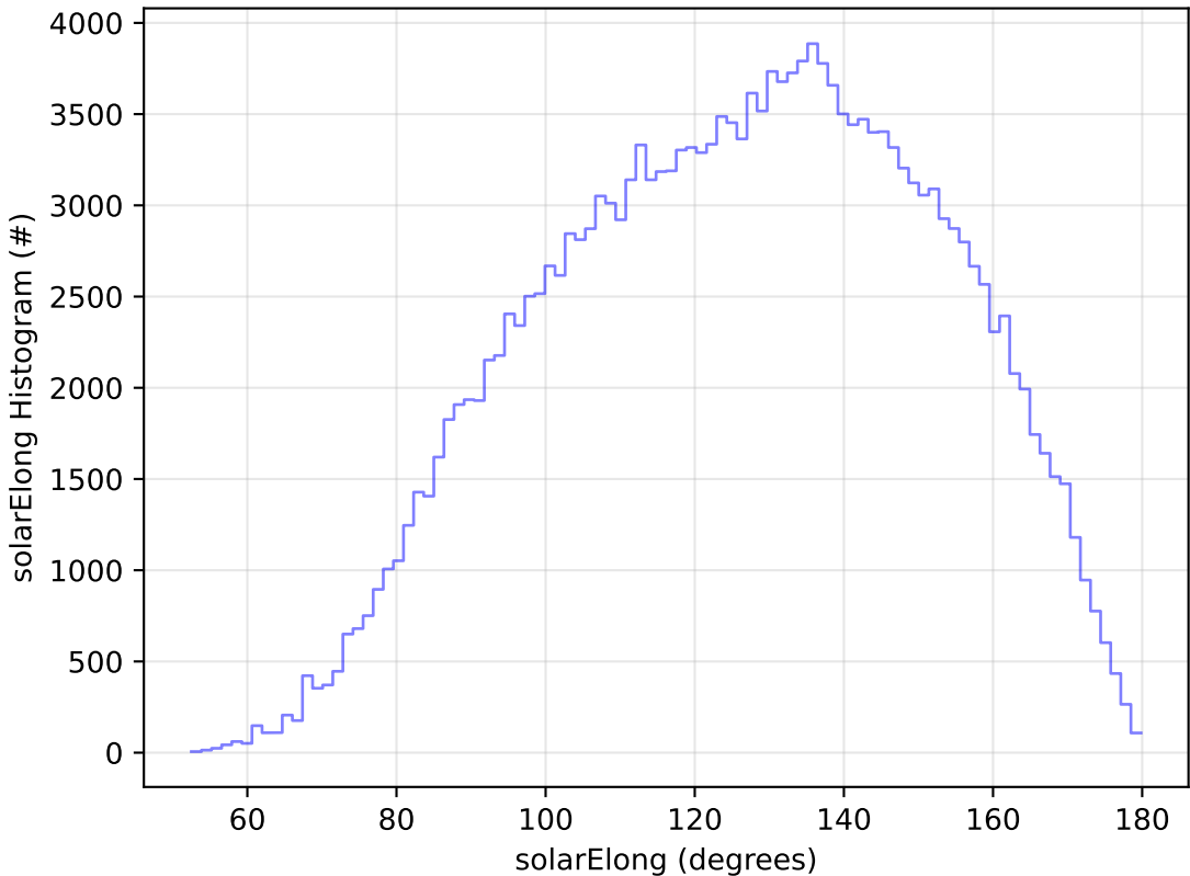
early_u_fpextra3.0_v3.4_10yrs All sky g band: solarElong Histogram
